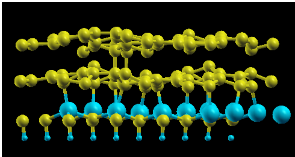
(A) H5.0-s1, C5.0-s1p1, Si7.0-s2p2d1
