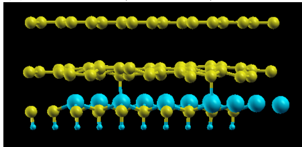
(B) H5.0-s2, C6.0-s2p2d1, Si7.0-s2p2d1
